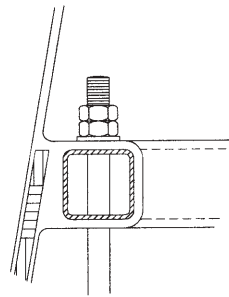
2 ANCHOR DETAIL
