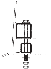
4 S1 BOLTING DETAIL
