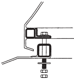
4 BOLTING DETAIL S1
