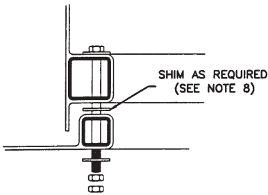
3 BOLTING DETAIL S1
