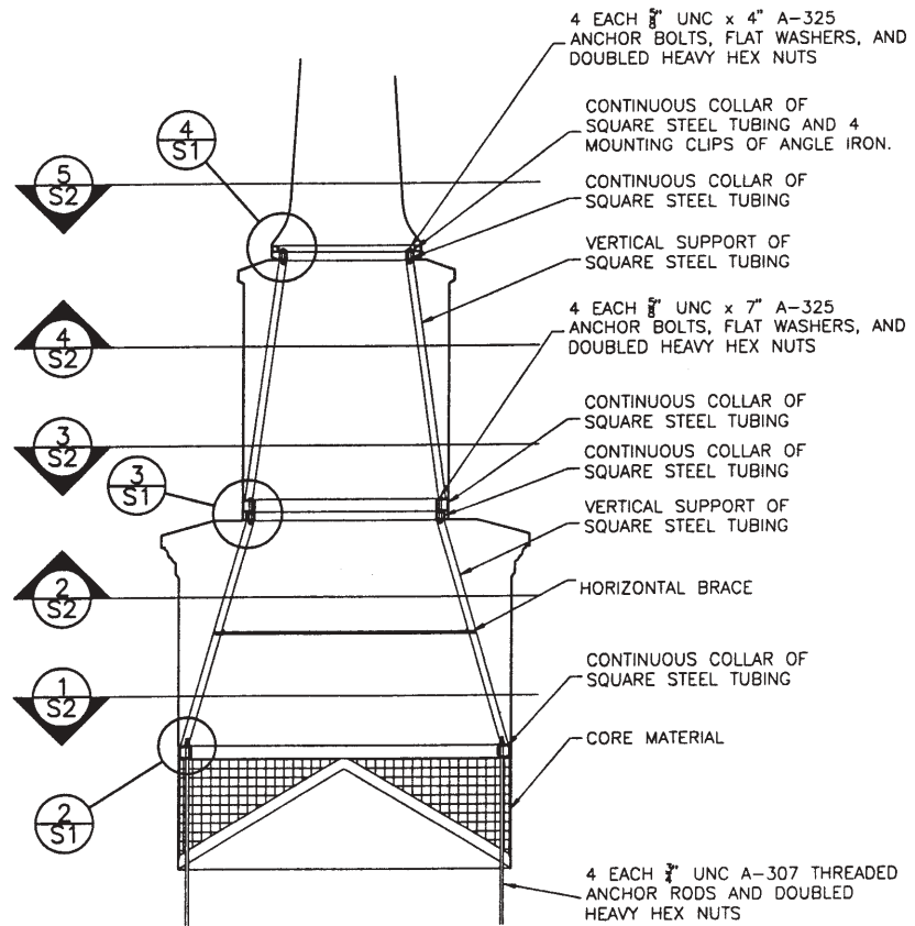
1 FULL SECTION S1
