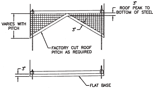
5 BASE DETAILS S1
