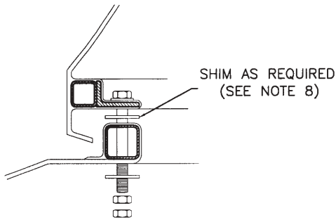
(2) BOLTING DETAIL S1
