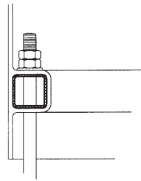
(3) ANCHOR DETAIL S1
