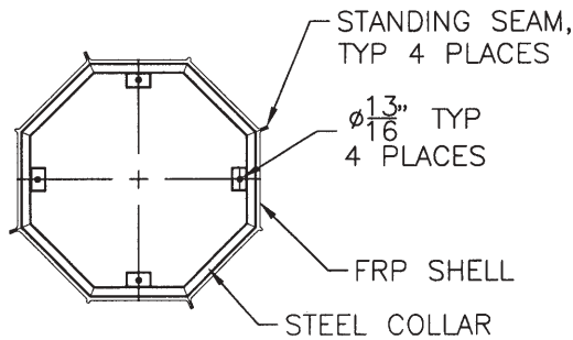
3 S2 BASE OF SP-619 PLAN VIEW
