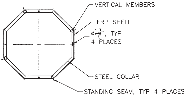
1 S2 BASE OF CU-601 PLAN VIEW
