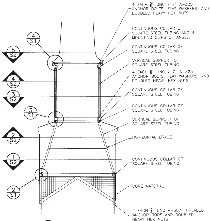
1 FULL SECTION S1
