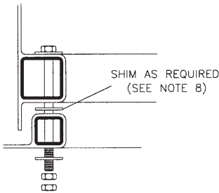
3 BOLTING DETAIL S1
