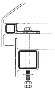
4 BOLTING DETAIL S1
